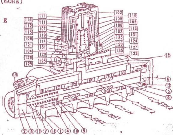
Fig. 1 Solenoid valve BN-7M43
